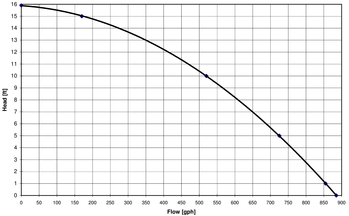
S900 Pump Curve Stainless steel / Brass
