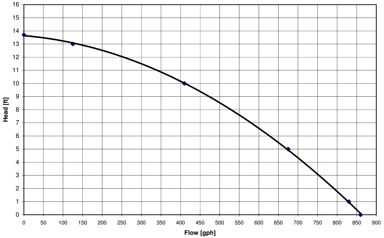
S580 Pump Curve Stainless steel / Brass
