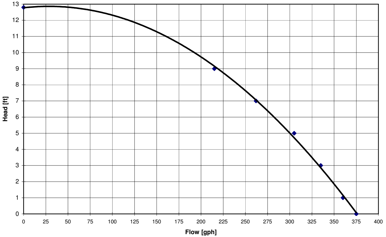
S320 Pump Curve Stainless steel / Brass
