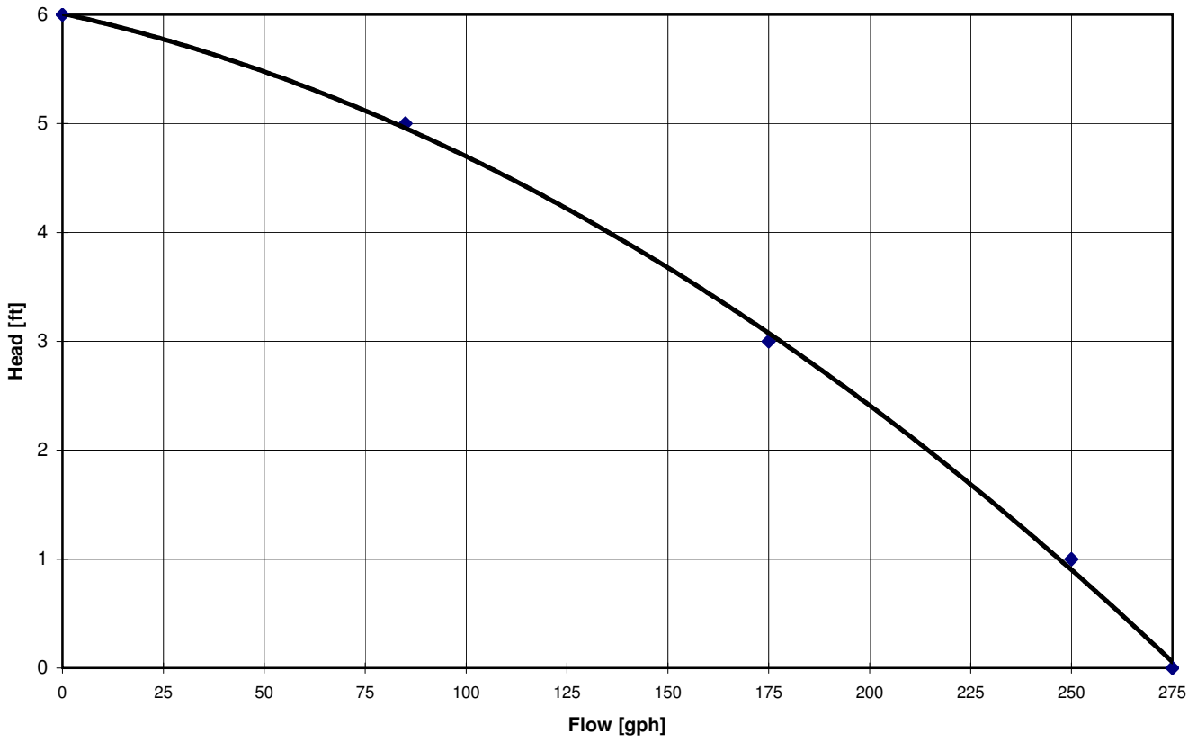
S225 Pump Curve Stainless steel / Brass
