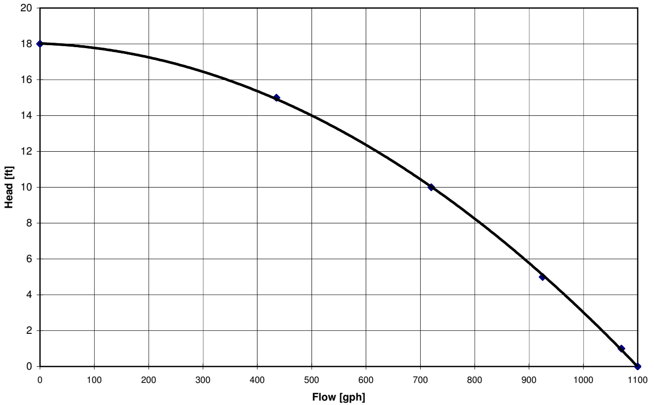
S1200 Pump Curve Stainless steel / Brass
