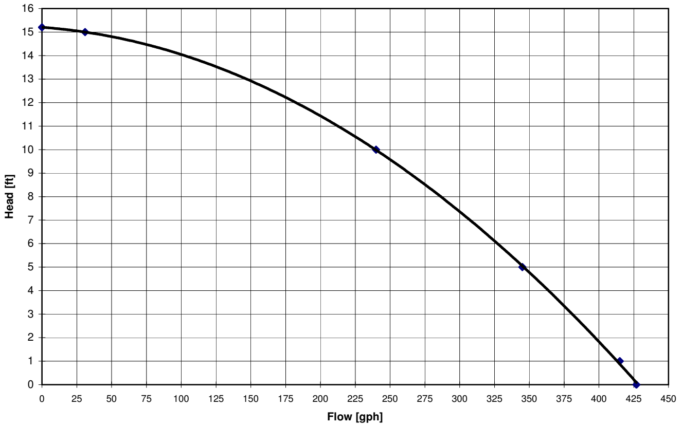
A430 Pump Curve Aluminum
