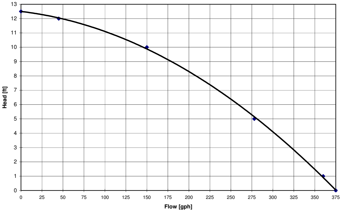
A280 Pump Curve Aluminum
