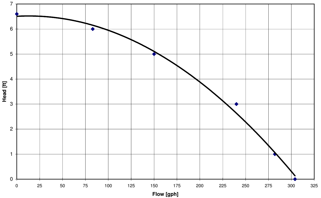
A210 Pump Curve Aluminum
